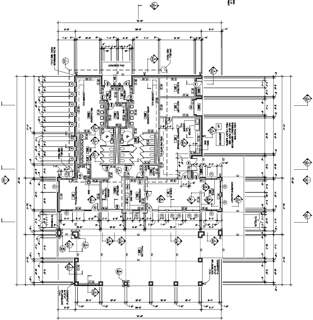
1 FLOOR PLAN - PRIMARY CONTROL BUILDING SCALE 3/8"=1'-0"
