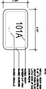
3 ROOM SIGN SCALE 3/8"=1'-0"
